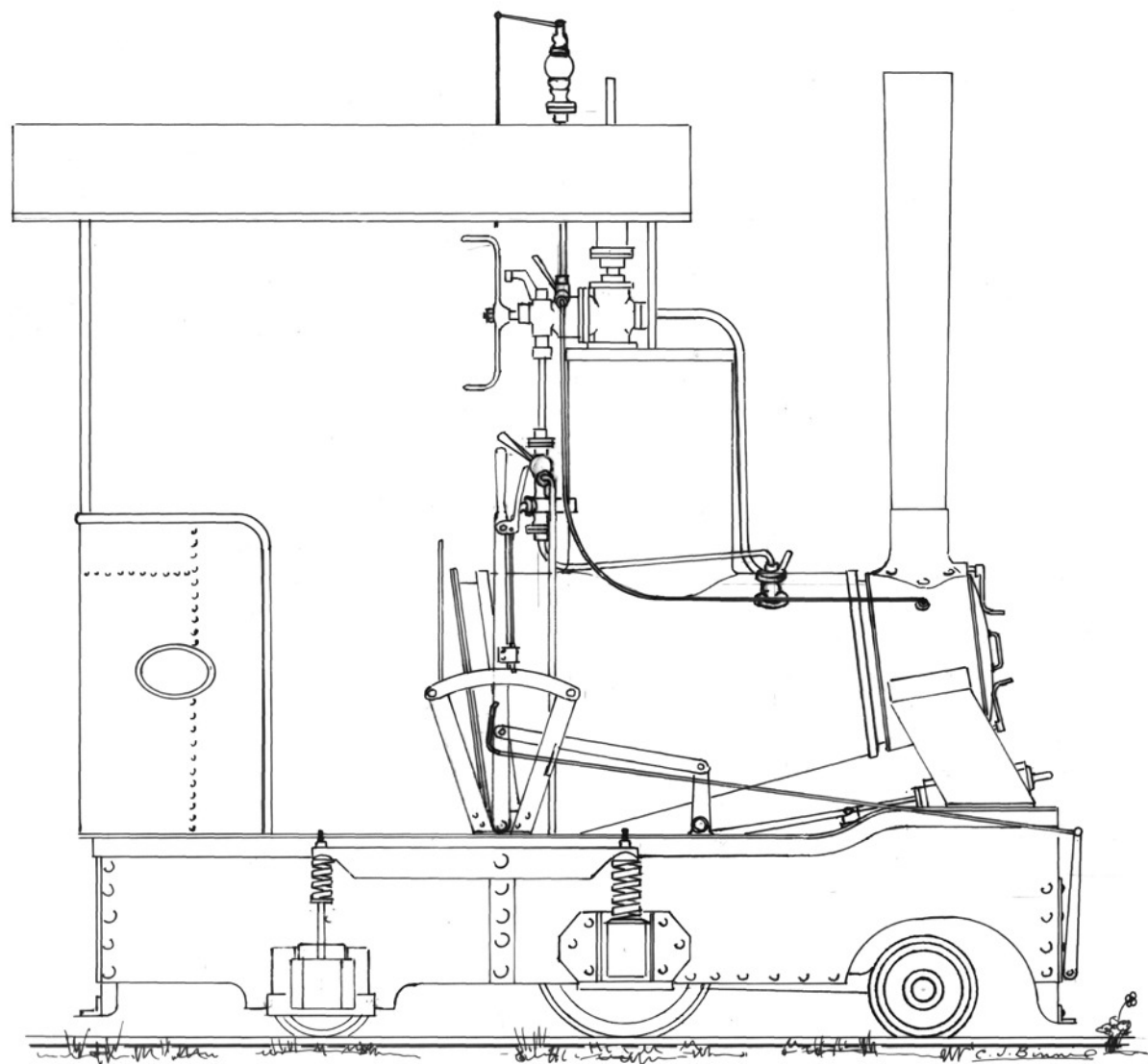
Hohenzollern 2-2-2 feldbahn lokomotive 447. Drawn from photograph by Colin Binnie
