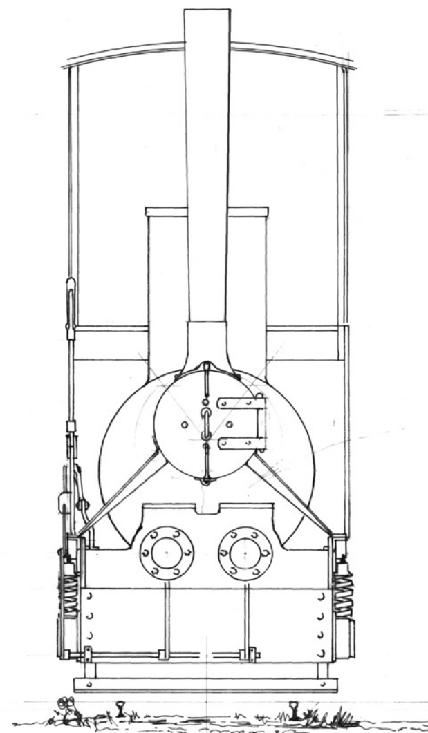
Hohenzollern 2-2-2 feldbahn lokomotive 447. Drawn from photograph by Colin Binnie
